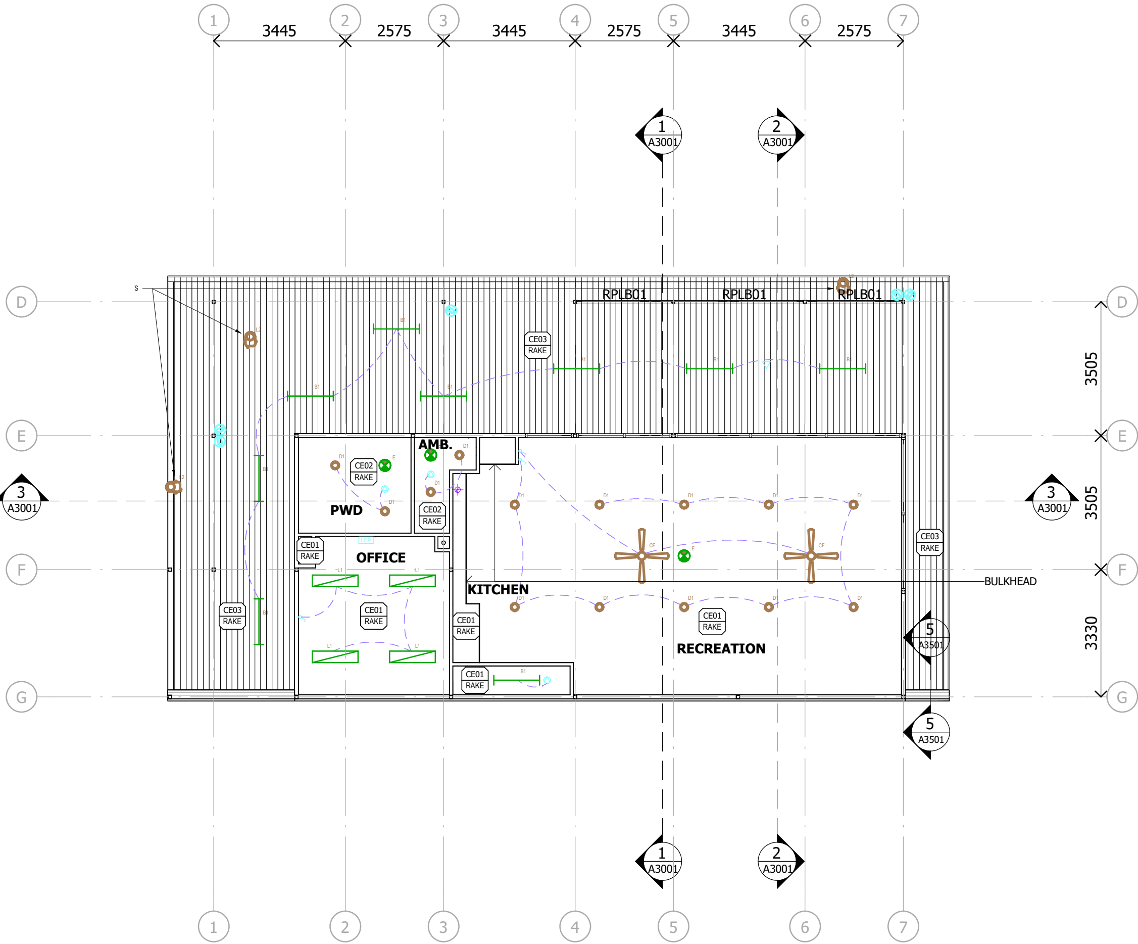
1 A2001 GROUND FLOOR - REFLECTED CEILING PLAN 1 : 100
